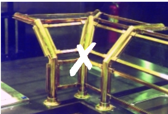
Out-dated Construction of clumsy round tube with applied channel The Results? Gaps, Food Traps, Unsound Structure, and Difficult to Clean.
